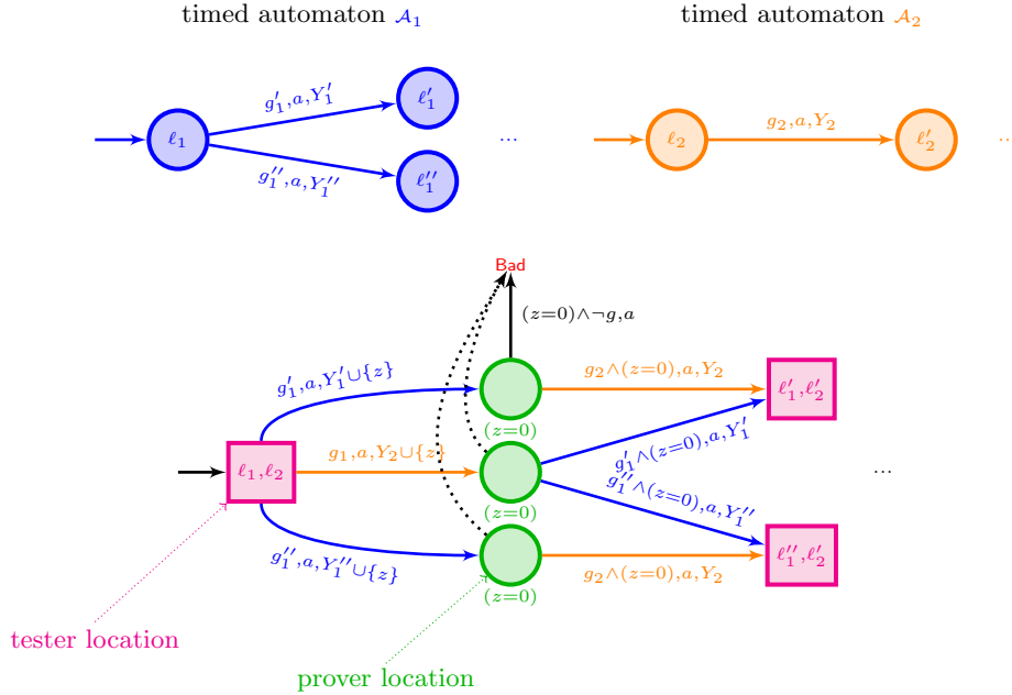
Fig. 9: Bisimulation game
