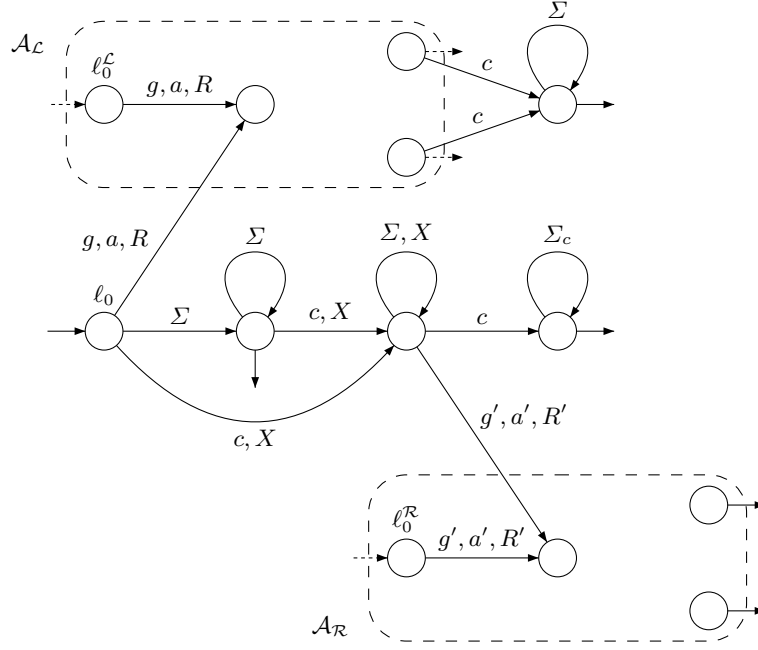
Fig. 3. Automaton recognizing the language \text{Compose}(\mathcal{L}, \mathcal{R}) .
