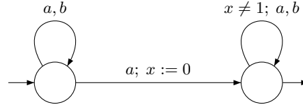
Fig. 4. The timed automaton accepting \mathcal{R}_{a,b}
