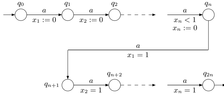
Fig. 5. Automaton \mathcal{A}_n with n clocks.
