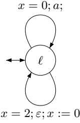
Fig. 1. A \text{TA}_\varepsilon not equivalent to any TA
