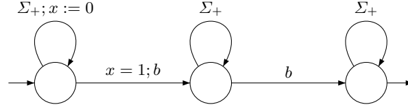
Fig. 6. A TA accepting \mathcal{W} .
