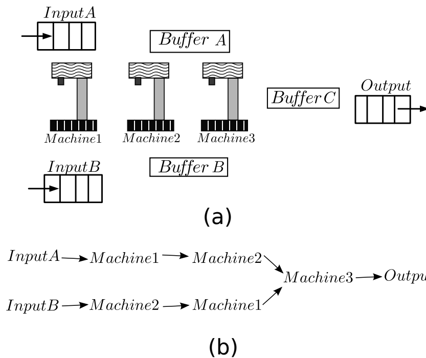
Figure 8. (a) Logical layout of a manufacturing system; and (b) its production process
